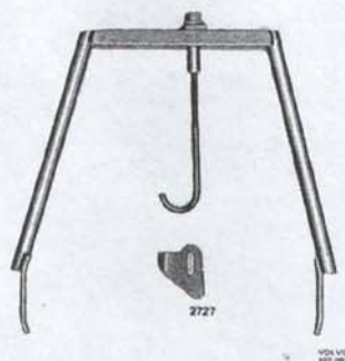
SVO 2727 Lifting tool for engine when removing sump and gearbox.
